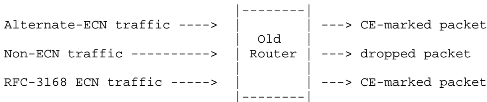
Figure 1: Alternate-ECN traffic, an old router, using RFC-3168 ECN, that is congested and ready to drop or mark the arriving packet.
