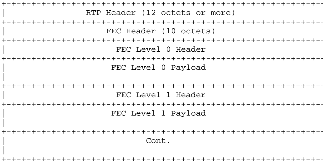
Figure 2: FEC Packet Structure
