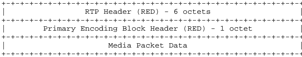
Figure 18: RED Packet Structure - Media Data Only
