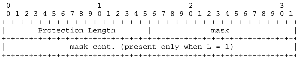
Figure 4: ULP Level Header Format
