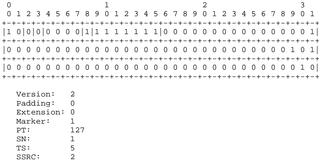
Figure 11: RTP Header of FEC Packet #1
