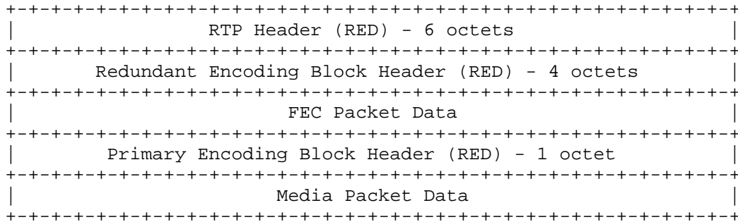
Figure 21: RED Packet Structure - With FEC Data
