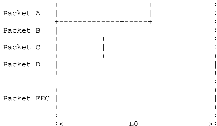
Figure 6: FEC Scheme with Single-Level Protection
