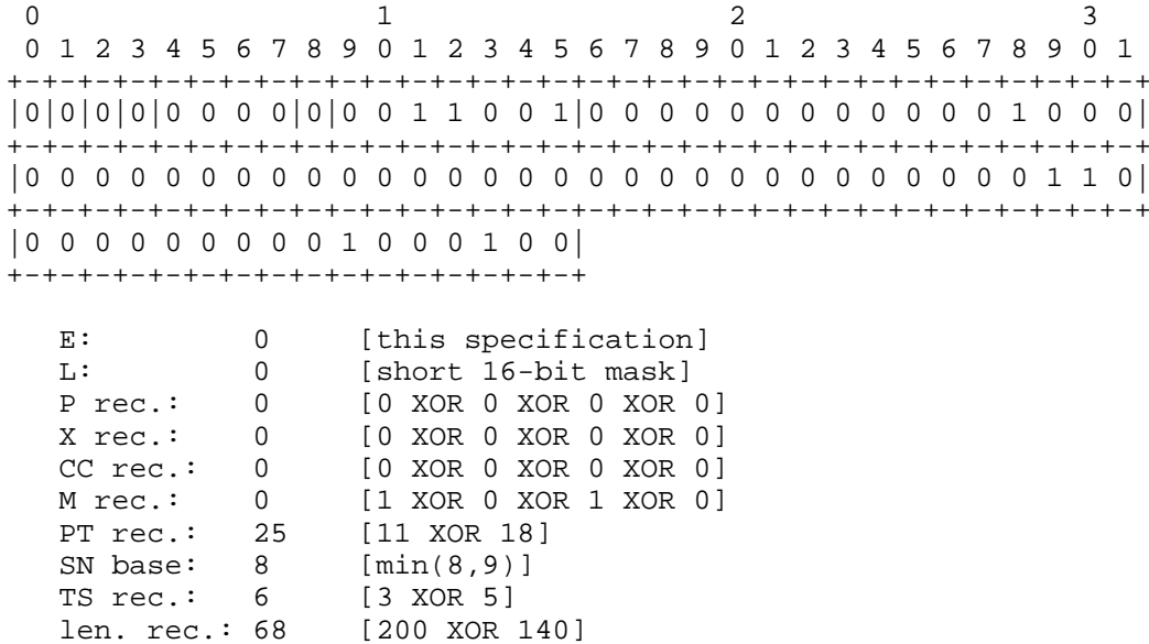
Figure 12: FEC Header of ULP FEC Packet #1
